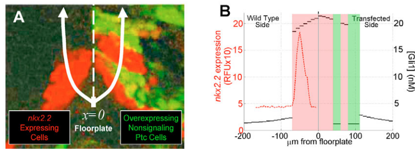
Fig. 3. Model predicts experimental patterning results. (A) A cross section of a stage 20-24 chick embryo indicates expression of nKx2.2 (red) and cells transfected with a signaling-defective Ptc (green) [adapted, with permission, from Briscoe et al. (Briscoe et al., 2001)]. (B) Modeling results of the Gli1 concentration in both the wild-type and transfected sides of the embryo after 63 hours of Shh secretion match experimental profiles. The dashed line indicates the experimentally measured Nkx2.2 profile at stage 18, t \approx 50 hours (Ericson et al., 1997b). See text for relationship between Nkx2.2 and Gli1. Simulation initial conditions and parameters are the same as those listed in Fig. 2, except within the transfected regions where (K_{ptc} K_{Gli3}) \geq 10^6 . See text for details.
