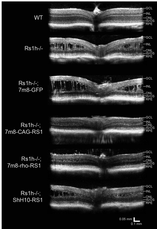
Figure 4. In vivo imaging of treated eyes 4 months after injection. Imaging of treated retinas showed that compared to WT mice, Rs1h -/- retinas were marked by the presence of large cavities in the superior and inferior retina. Similarly, 7m8-GFP-treated eyes were highly disorganized with large cavities. In comparison, 7m8-CAG-RS1 and 7m8-rho-RS1 retinas had fewer and smaller holes. ShH10-RS1-injected eyes were also marked by the presence of cavities. For each treatment group, n = 5 animals were imaged.
