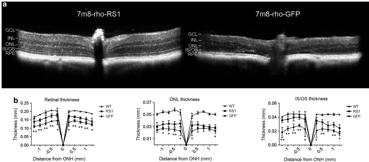
Figure 5. In vivo imaging of long-term structural rescue. (a) Spectral domain optical coherence tomography images of 7m8-rho-RS1- or 7m8-rho-GFP-treated retinas 10 months post-injection showed improved retinal structure in 7m8-treated eyes. (b) Measurements of retinal thickness, ONL thickness and inner and outer segment thickness showed increased thickness in 7m8-rho-RS1-treated retinas in superior and inferior portions of the retina. Asterisks indicate statistical significance of the difference between treated and untreated eyes at the eccentricity measured as determined by a paired two-tailed Student's t -test. * P < 0.05, ** P < 0.01. n = 5 for each condition. Error bars are mean ± s.d.
