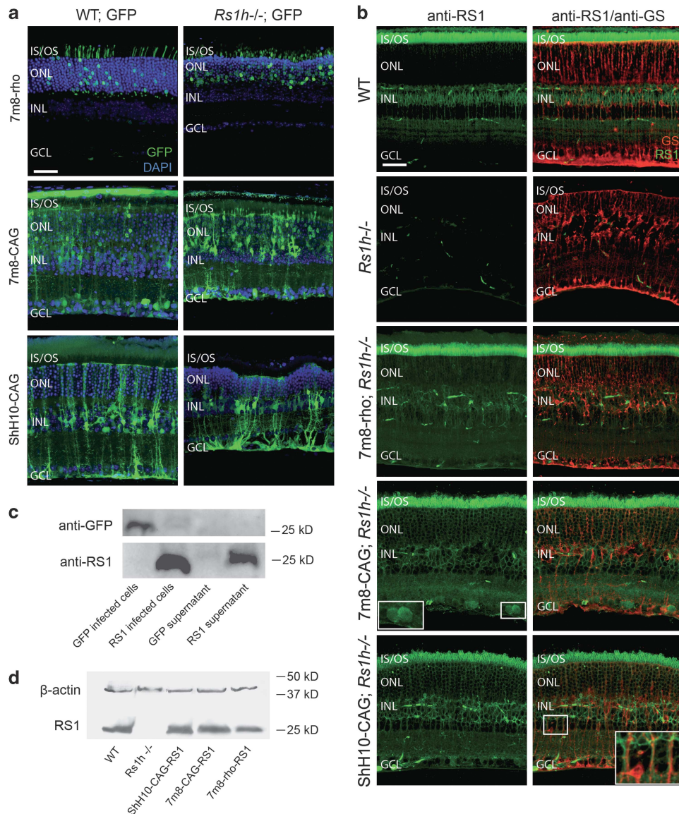
Figure 2. Characterization of viral vectors. (a) GFP expression in WT and Rs1h -/- retinas 4 months after intravitreal injection of viral vectors shows the cell types targeted. 7m8-rho-GFP leads to expression specifically in photoreceptors. 7m8-CAG-GFP leads to the expression in all retinal layers. ShH10-CAG-GFP specifically expresses in Müller glia. Blue is 4,6-diamidino-2-phenylindole-labeled nuclei. Green is native GFP expression. (b) Expression of RS1 4 months after intravitreal injection of the three vectors. First row: labeling of retinoschisin in the WT retina shows localization in inner segments of photoreceptors, bipolar cells and the photoreceptor-bipolar cell synapse, while Rs1h -/- retinas (second row) are devoid of the protein. Third row: 7m8-rho-RS1 injection in Rs1h -/- mice leads to strong expression of the protein with localization of the protein like in the WT retina. Fourth row: 7m8-CAG-RS1 leads to similar levels of protein expression in inner segments and the inner plexiform layer, although the protein is also expressed from Müller cells and ganglion cells. Inset shows magnification of RS1 expression in ganglion cell bodies. Fifth row: ShH10-CAG-RS1 injection in Rs1h -/- mice leads to RS1 protein localization in all retinal layers, including inner segments of photoreceptors, although the staining in photoreceptors was less strong than with the 7m8 vectors. Inset shows detail of RS1 staining on bipolar cell processes running parallel to Müller glia. Red is labeling of the Müller cell marker glutamine synthetase (GS). Green is labeling of RS1. (c) Mouse Müller cells infected with ShH10-RS1 secrete RS1. Primary Müller cell cultures were infected with ShH10-GFP or ShH10-RS1. GFP was present only in cell lysate from cells infected with ShH10-GFP, but not in culture media or in cells infected with ShH10-RS1 (top row). RS1, in contrast, was secreted and was found in both cell lysate and culture media (bottom row). (d) A western blot from retinas injected with ShH10, 7m8-CAG or 7m8-rho shows that levels of expression are similar to WT following treatment with all three vectors. GCL, ganglion cell layer; INL, inner nuclear layer; IS/OS, inner and outer segments; ONL, outer nuclear layer.
