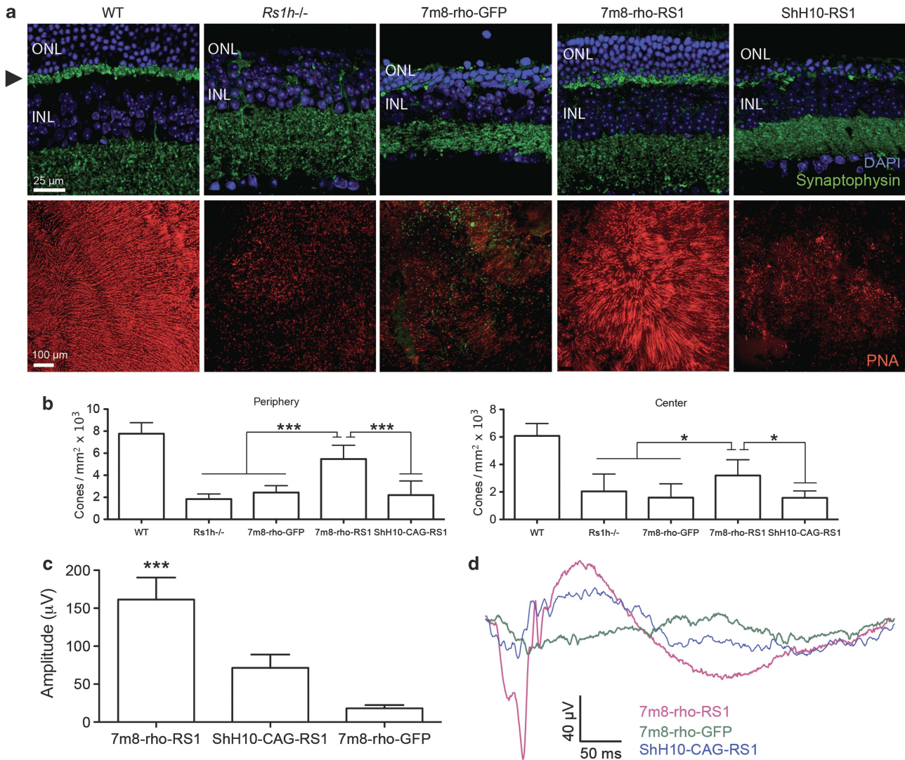
Figure 6. Long-term structural and functional rescue. (a) Retinas collected from mice 15 months post-injection and labeled with anti-synaptophysin antibodies showed that the structure of the photoreceptor – bipolar cell synapse was maintained in mice injected with 7m8-rho-RS1, and looked more like WT compared to untreated Rs1h -/- eyes or control 7m8-GFP-injected eyes. ShH10-RS1-injected eyes also showed synaptic deterioration. Peanut agglutinin labeling, which labels cones, showed that the population of structurally intact cones in Rs1h -/- mouse retinas is nearly eliminated by 15 months after birth. Mouse eyes treated with 7m8-rho-RS1 showed a much improved cone histology, with widespread labeling of surviving cones. However, at this time point ShH10-injected eyes showed no cone preservation compared to control eyes. (b) Quantification of cone labeling in peripheral and central retina showed that 7m8-rho-RS1-treated eyes had significantly greater number of cones compared with untreated or control eyes ( n = 5 for each group). ShH10-treated eyes ( n = 5 ) had similar number of cones compared to untreated eyes. (c) ERGs recorded 15 months after injection showed preservation of the b-wave in 7m8-rho-RS1-treated eyes compared to 7m8-rho-GFP-treated eyes or ShH10-CAG-RS1-treated eyes ( n = 5 per group). (d) Representative ERG traces show that 7m8-rho-RS1-treated eyes had a more normal wave form and a higher amplitude of the a- and b-waves compared with ShH10 or contralateral control eyes. Error bars are mean \pm s.d. *** P < 0.001 , * P < 0.05 .
