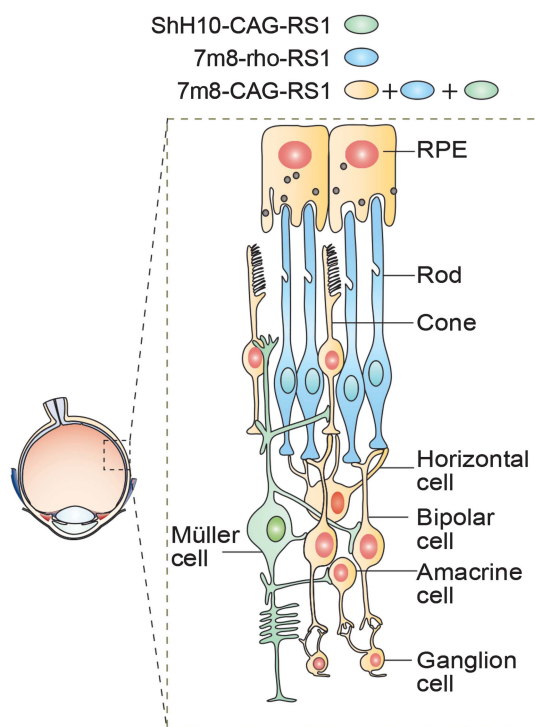
Figure 1. Illustration of experimental plan. Three vectors were used to deliver RS1 to specific population of retinal cells following intravitreal injection. ShH10 targets Müller glia (in green), which contact all retinal neurons and span the retina from the inner-limiting membrane to the outer-limiting membrane. 7m8 with a rhodopsin promoter specifically expresses in photoreceptors (in blue). 7m8 with a ubiquitous CAG promoter penetrates to the outer retina from the vitreous and infects all retinal cell types (orange), including ganglion cells, photoreceptors and Müller glia.
